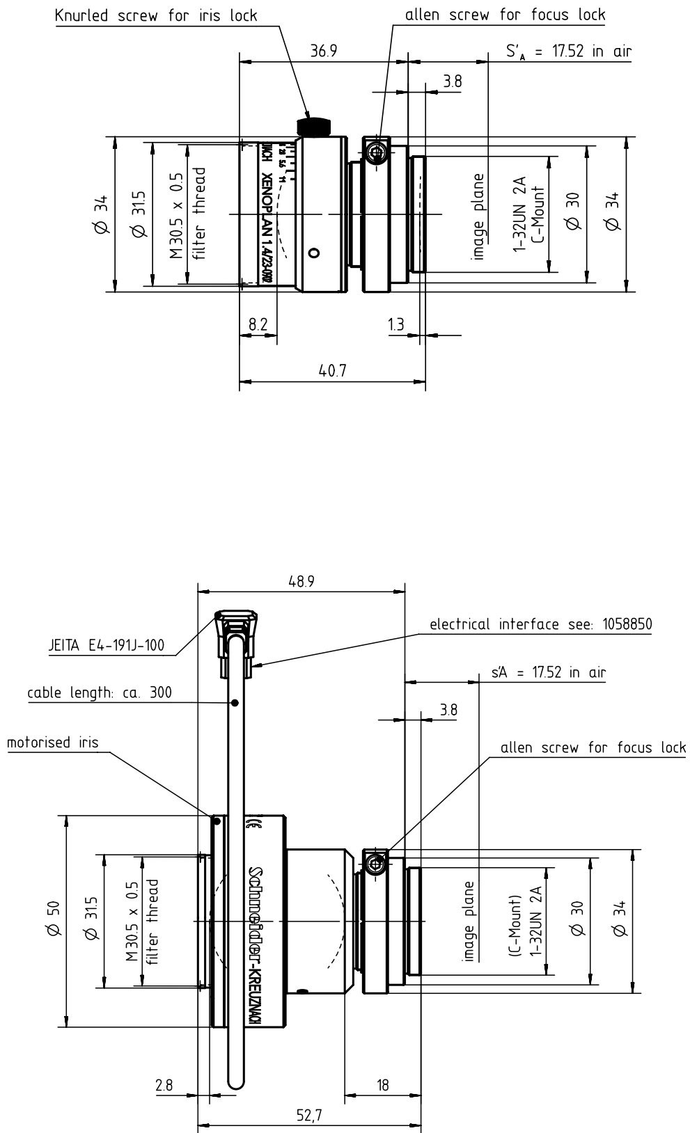
Motorized p-iris
